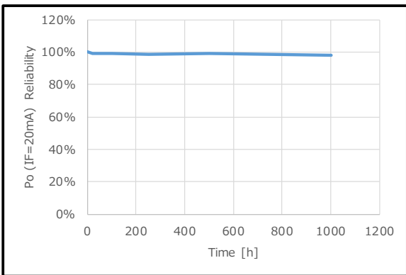
Figure 12. 85°C,85% 50mA 1,000h test
