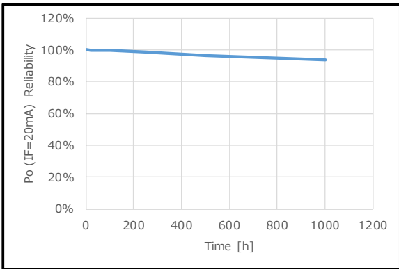
Figure 11. 100°C 50mA 1,000h test
