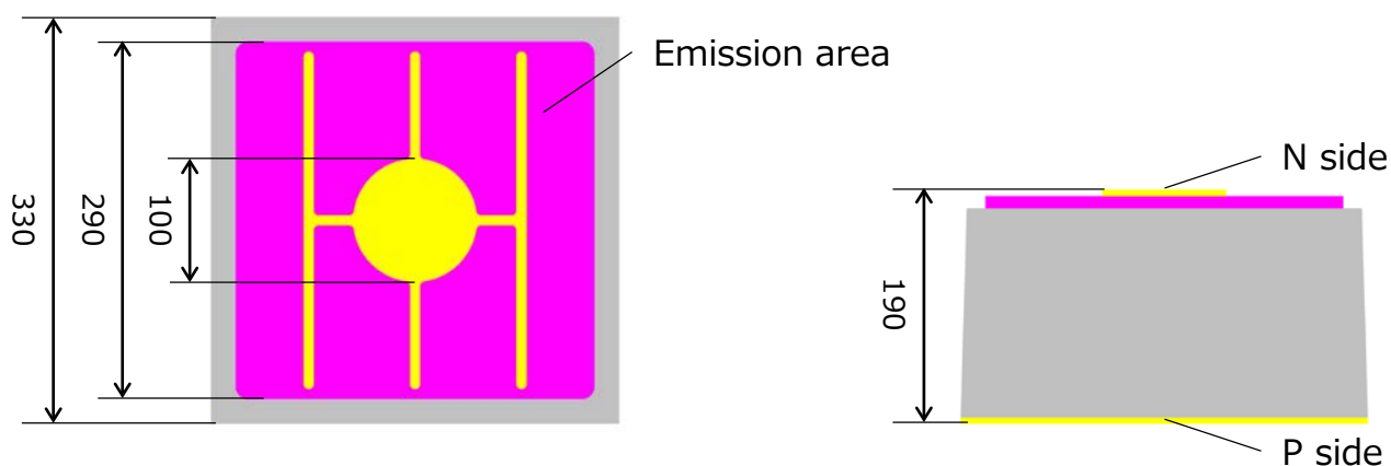
Figure 1. Electrode pattern and Chip size (Unit : \mu\text{m} )
